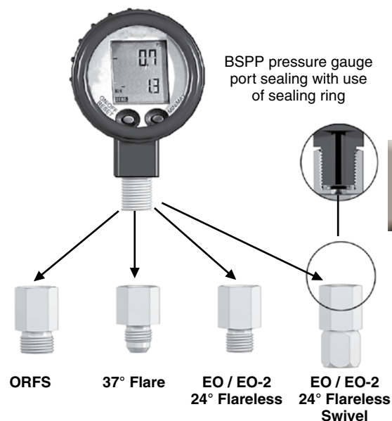
Fig. M4 — BSPP pressure gauge connections
