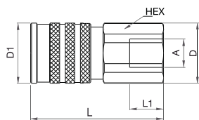
Female Thread
