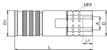
PE Female Thread
