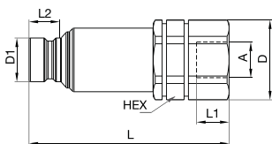
PE Female Thread
